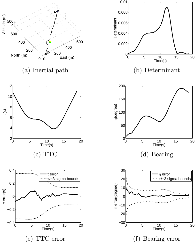
Figure 6: This figure shows the simulation results for single obstacle avoidance problem. Subfigure (a) shows the inertial path. Subfigure (b) shows the determinant of \mathbf{O}^i \mathbf{O}^i . Subfigures (c) and (d) show the TTC and bearing to the obstacle. Subfigure (e) and (f) show the estimation error and \pm 3\sigma bounds of the error covariance for the TTC and bearing.
