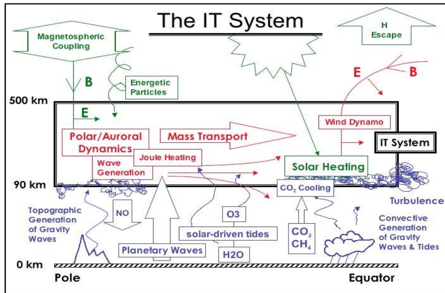
Figure 1: Thermosphere Heating and Dynamics Processes.
