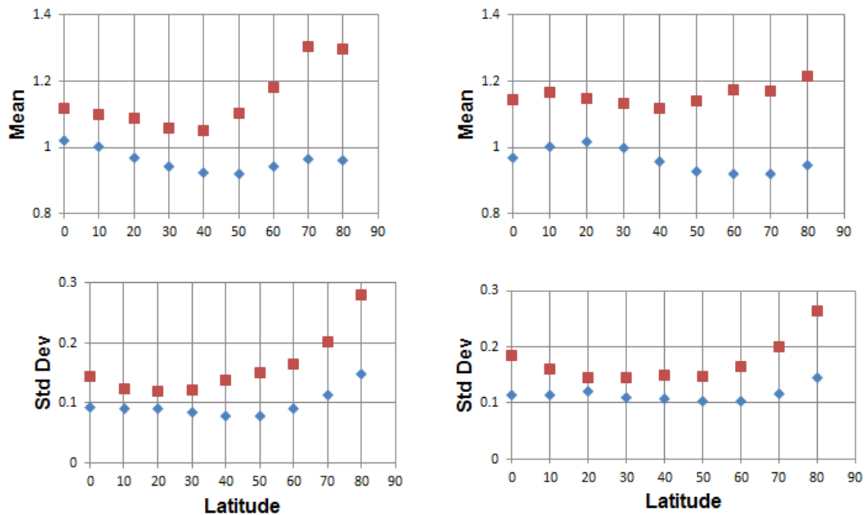
Figure 20a: SETA-2 to TIEGCM ratios vs latitude for northern hemisphere data in two ap bins, 0-10 (blue) and >100 (red). Left: daytime local times; Right: nighttime local times
