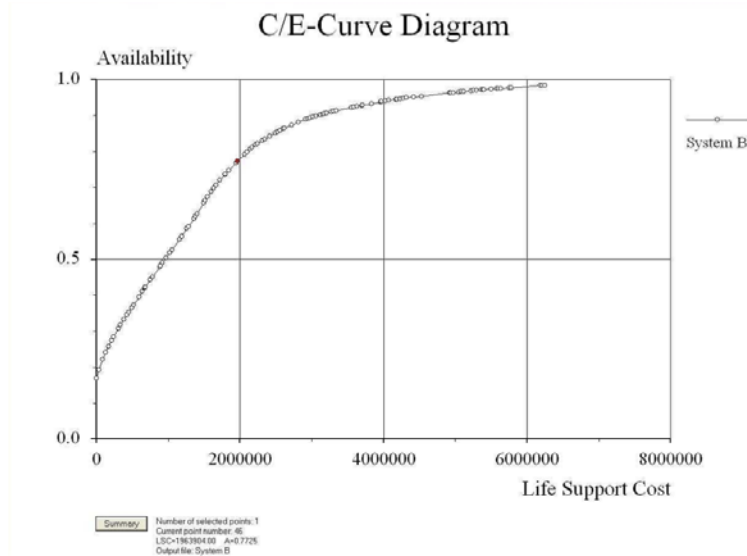
Figure 2-2. OPUS10 Sample Cost-Effectiveness (Availability vs Cost) Curve
