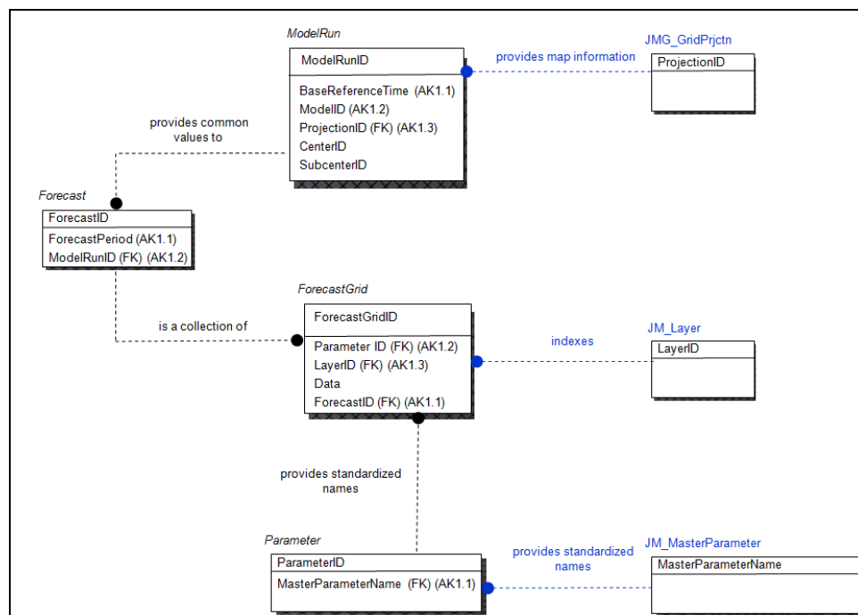
Figure 2. GMDB schema.
