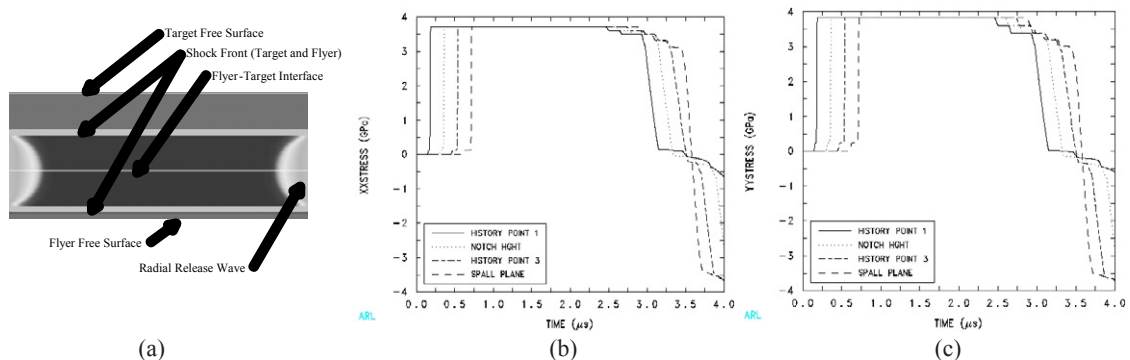
Fig. 3. (a) Simulation result for the baseline case with no notch at 1 \mu s, (b) and (c) are the resulting stress-time histories for various tracer locations up to 4 \mu s.
