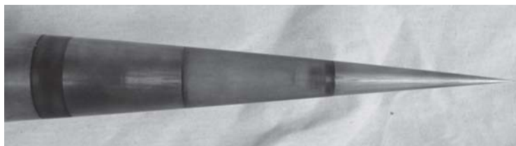
Figure 1. Top: Aluminum cone, 1m in length, instrumented with 80 thermocouples in 20 rows. Bottom, from right to left: molybdenum tip, plastic holder with 316L stainless steel 10 micron porous section, aluminum cone body.
