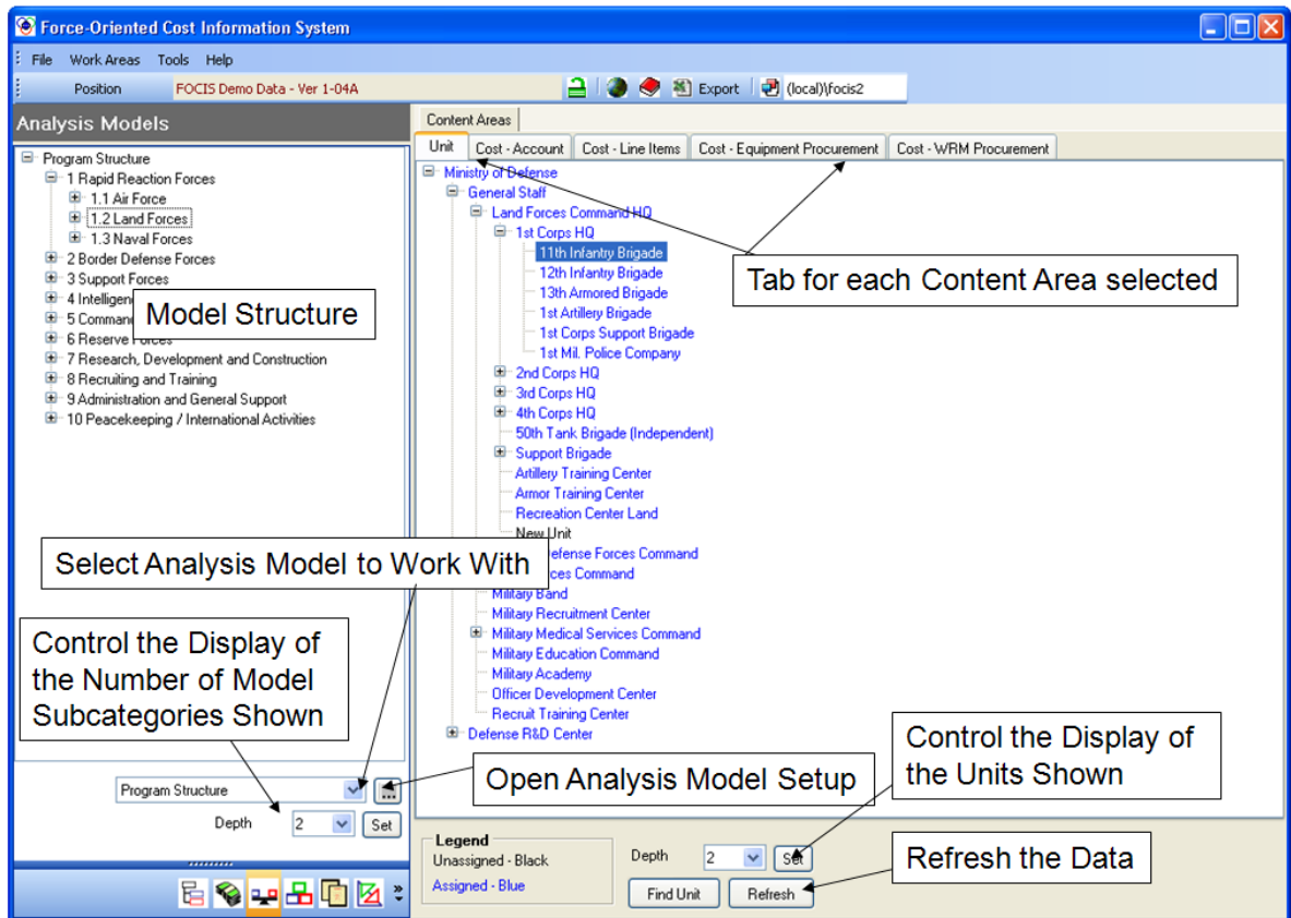
Figure 6-19. Analysis Models Work Area Window
