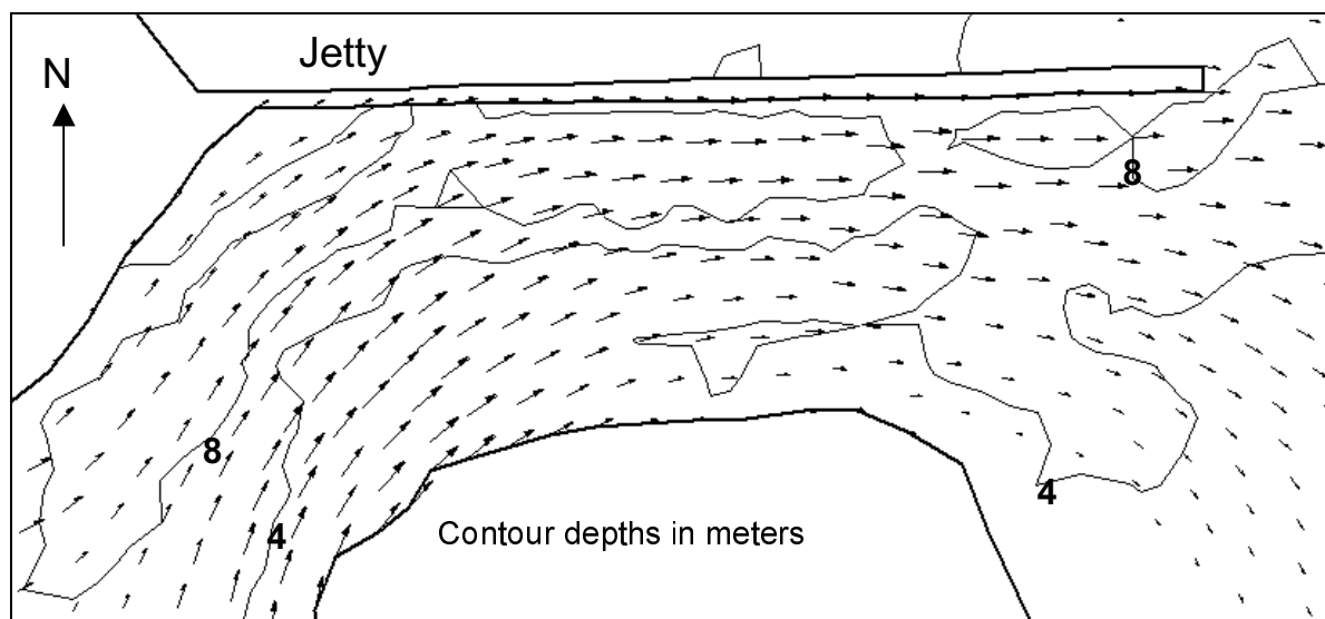
Figure 1. Calculated current vectors in Ponce De Leon Inlet, Florida, overlain on depth contours (4-m intervals)
