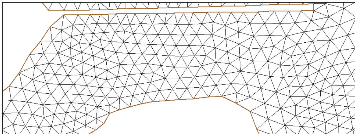
Figure 3. Detail of finite-element mesh in inlet, Ponce De Leon Inlet, Florida
