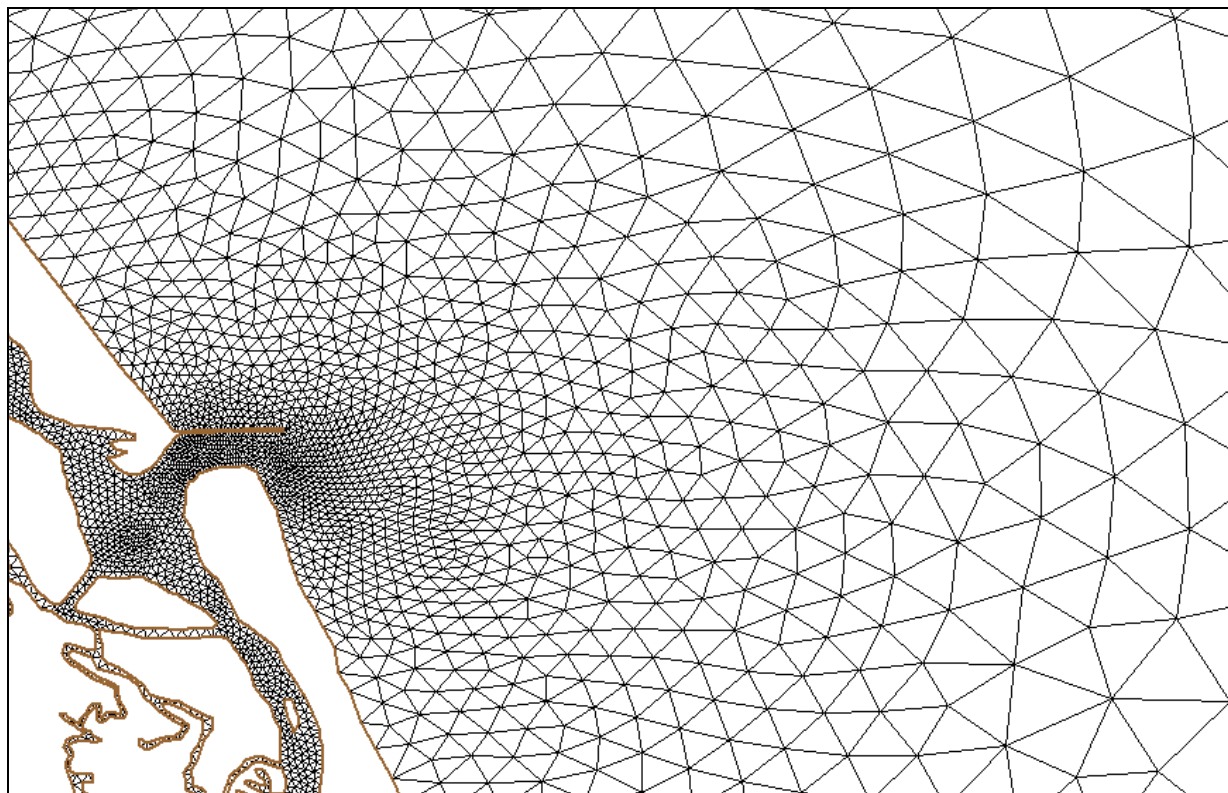
Figure 2. Graded finite-element mesh, Ponce De Leon Inlet, Florida
