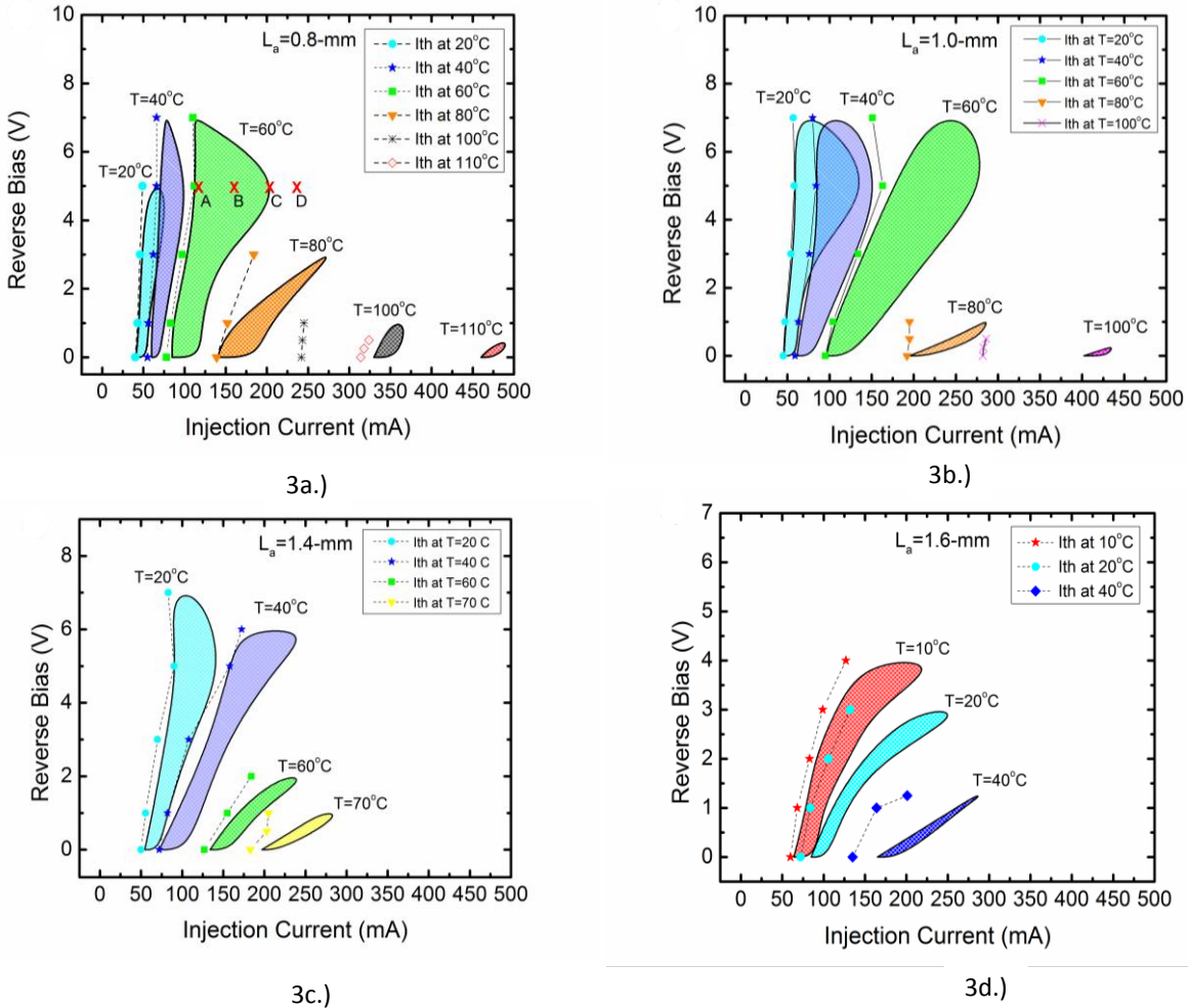
Fig. 3. Contour maps depicting the regions of fundamental mode-locking (5 GHz) where the measured FWHM of the optical pulse was less than 19 ps for a.) L_a=0.8\text{-mm} , b.) L_a=1.0\text{-mm} , c.) L_a=1.4\text{-mm} , and d.) L_a=1.6\text{-mm} . These absorber lengths are depicted in the modeled mode-locking stability maps in Figs. 2a.) and 2b.). The plotted symbols show the threshold current at each temperature and reverse voltage.
