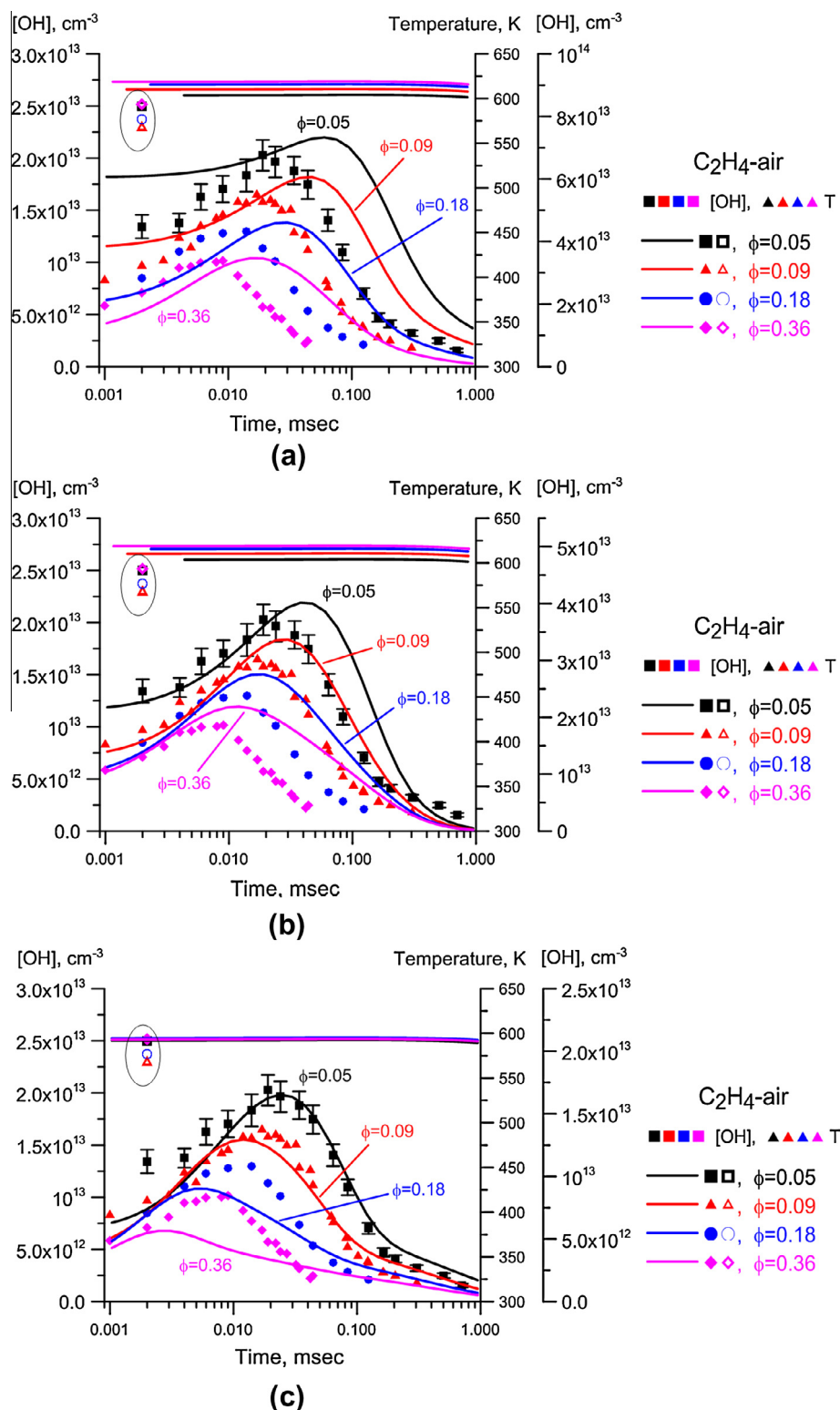
Fig. 16. Comparison of experimental and predicted time-resolved, absolute OH number densities after a \nu = 10 kHz, 50-pulse discharge burst in \text{C}_2\text{H}_4 -air mixtures at T_0 = 500 K, P = 100 torr, and different equivalence ratios. Data points for temperatures measured at the end of the burst (time delay 2 \mu\text{s} ) are circled. (a) GRI 3.0 mechanism, (b) USC/Wang mechanism and (c) Konnov mechanism.
