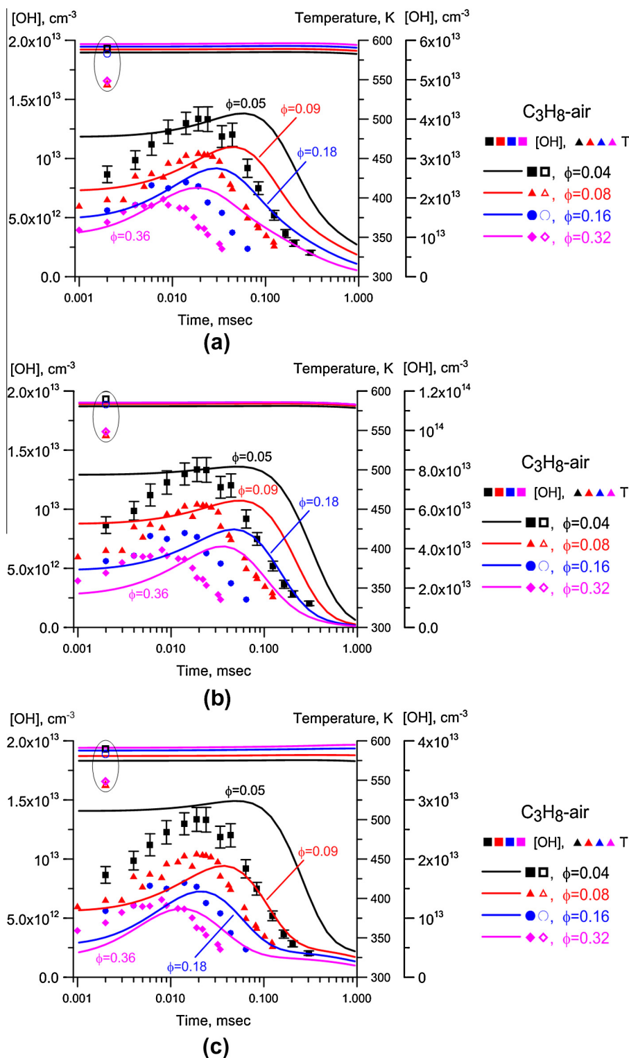
Fig. 17. Comparison of experimental and predicted time-resolved, absolute OH number densities after a \nu = 10 kHz, 50-pulse discharge burst in \text{C}_3\text{H}_8 -air mixtures at T_0 = 500 K, P = 100 torr, and different equivalence ratios. Data points for temperatures measured at the end of the burst (time delay 2 \mu\text{s} ) are circled. (a) GRI 3.0 mechanism, (b) USC/Wang mechanism and (c) Konnov mechanism.
