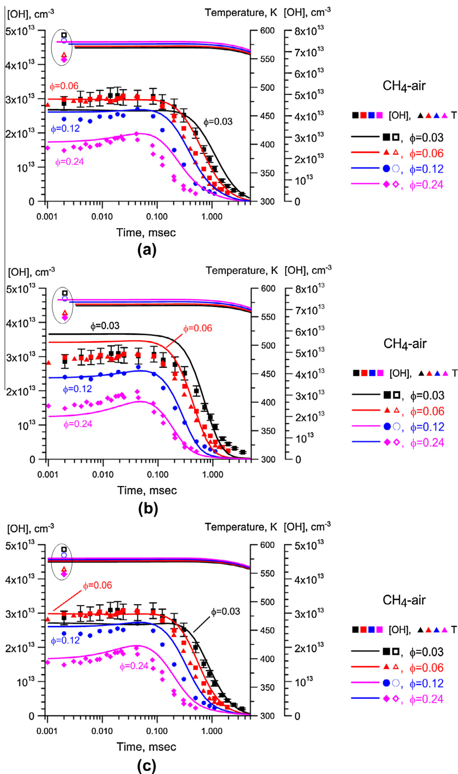
Fig. 15. Comparison of experimental (y-axis on the left) and predicted (y-axis on the right) time-resolved, absolute OH number densities after a \nu = 10 kHz, 50-pulse discharge burst in \text{CH}_4 -air mixtures at T_0 = 500 K, P = 100 torr, and different equivalence ratios. Data points for temperatures measured at the end of the burst (time delay 2 \mu\text{s} ) are circled. (a) GRI 3.0 mechanism, (b) USC/Wang mechanism and (c) Konnov mechanism.
