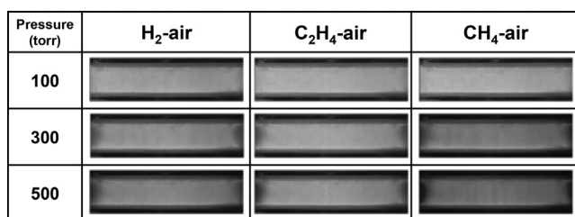
Fig. 6. Single shot ICCD images of the plasma in fuel–air mixtures illustrating discharge uniformity. T_0 = 500 K, \phi = 0.3 , \nu = 10 kHz, pulse #10. Camera gate = 50 ns.
