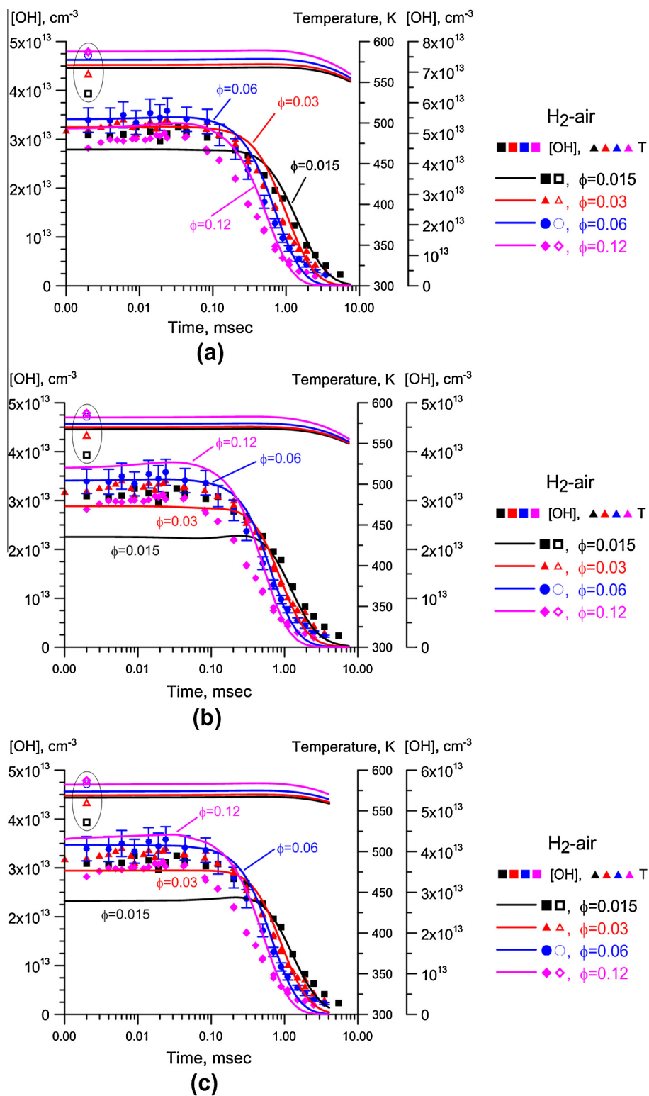
Fig. 14. Comparison of experimental (y-axis on the left) and predicted (y-axis on the right) time-resolved, absolute OH number densities after a \nu = 10 kHz, 50-pulse discharge burst in \text{H}_2 -air mixtures at T_0 = 500 K, P = 100 torr, and different equivalence ratios. Data points for temperatures measured at the end of the burst (time delay 2 \mu\text{s} ) are circled. (a) Popov mechanism, (b) Konnov mechanism and (c) Konnov mechanism with modified rate of reaction \text{OH} + \text{O} \rightarrow \text{H} + \text{O}_2 .
