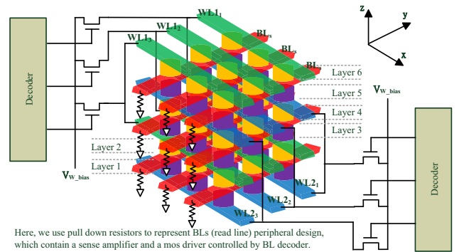
Fig. 2. 3D-HIM structure.
