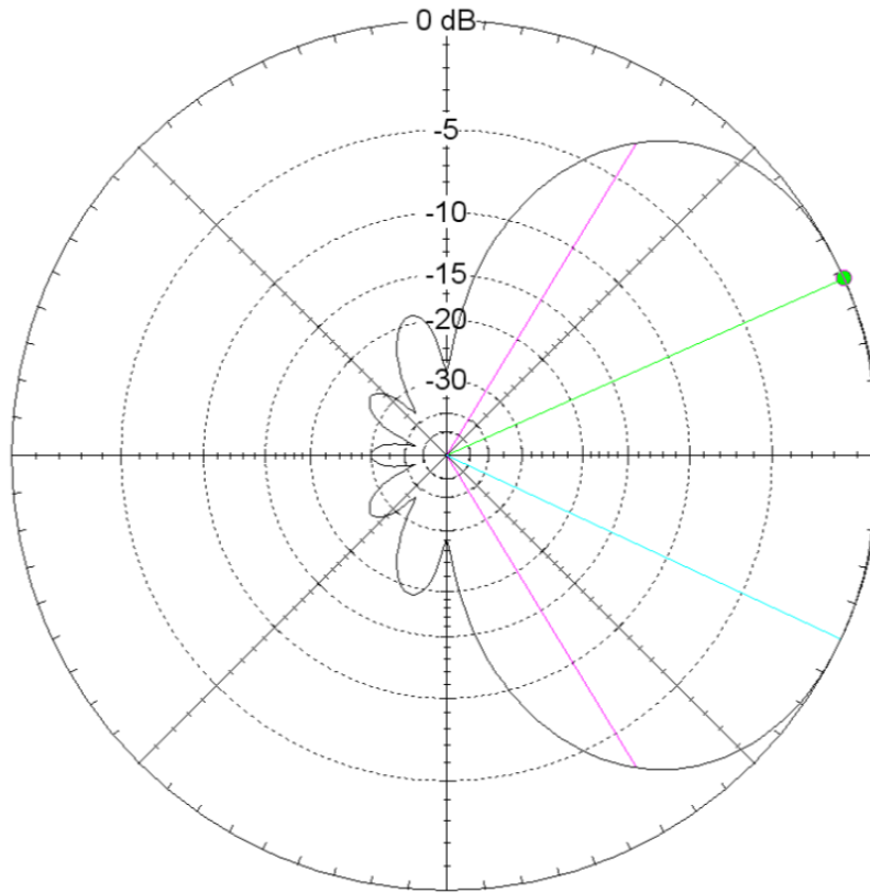
Figure 13. Surface wave of the directional antenna at 1 km and the 0-dB reference level is -9.63 dB.
