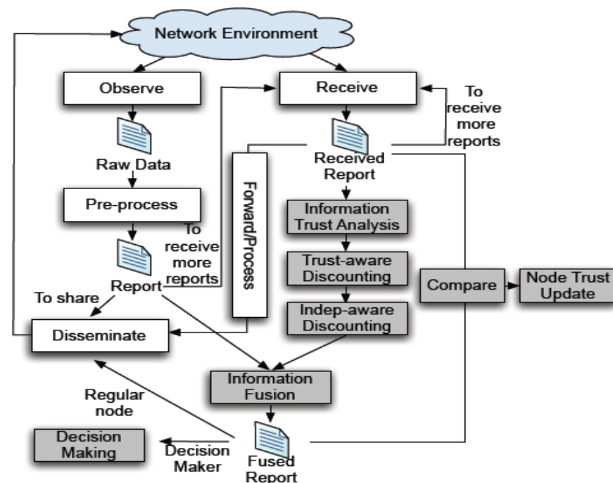
Node operations for decision making
