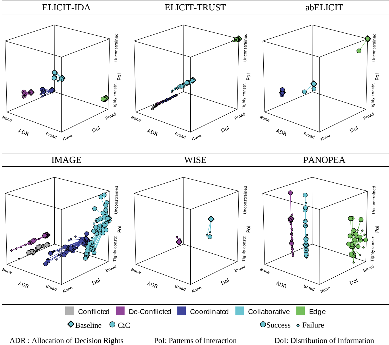
Figure 3: Tri-dimensional mapping of the endeavour space (CiCs) into the C2 Approach Space.
