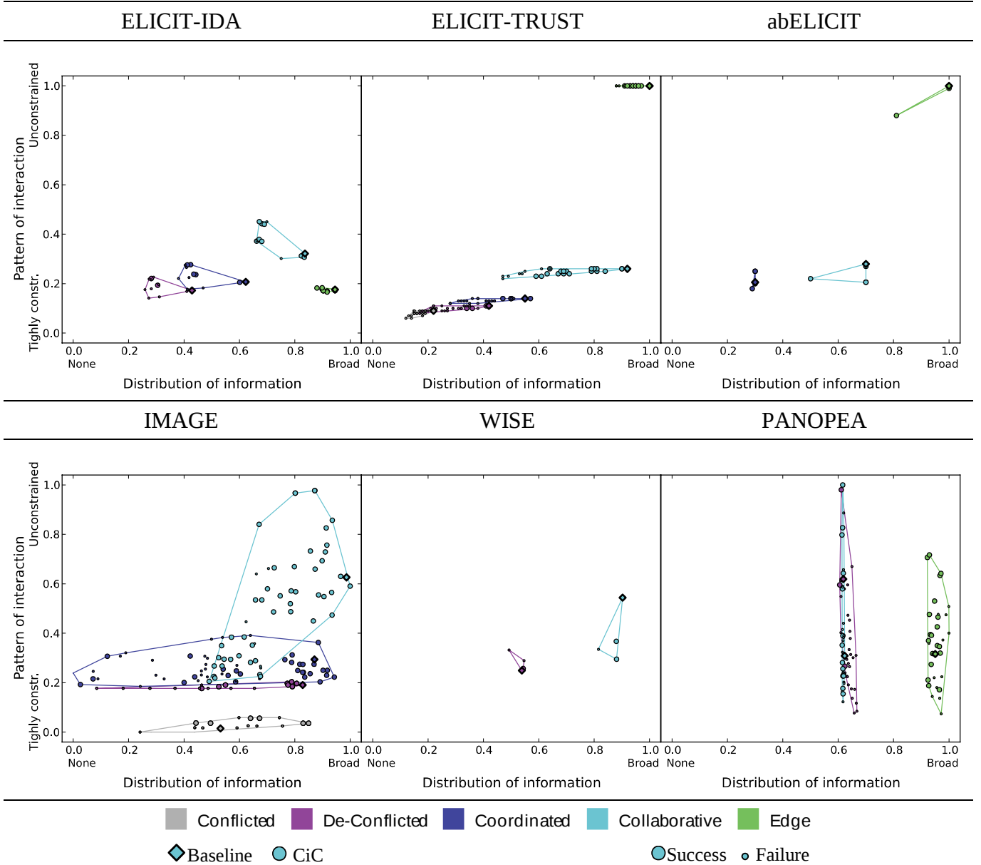
Figure 4: Spreading in the DoI-PoI plane according to each experiment and C2 Approach.
