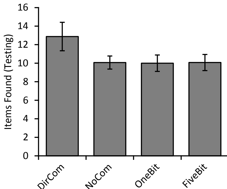
Figure 5: Test performance. The testing performance of a single run is determined by the average number of food items collected over 10,000 trials by the team with the highest training performance. Results for each communication scheme are averaged over 20 runs. Error bars depict a 95% confidence interval. The DirCom scheme performs significantly better than the other schemes ( p < 0.05 ; Student’s t-test).
