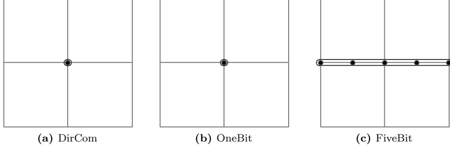
Figure 3: Substrate: communication output planes. The number of neurons on the communication output plane corresponds to the size of the signal vector sent to all other agents on the team on each tick: one for DirCom (a) and OneBit (b), and five for FiveBit (c).
