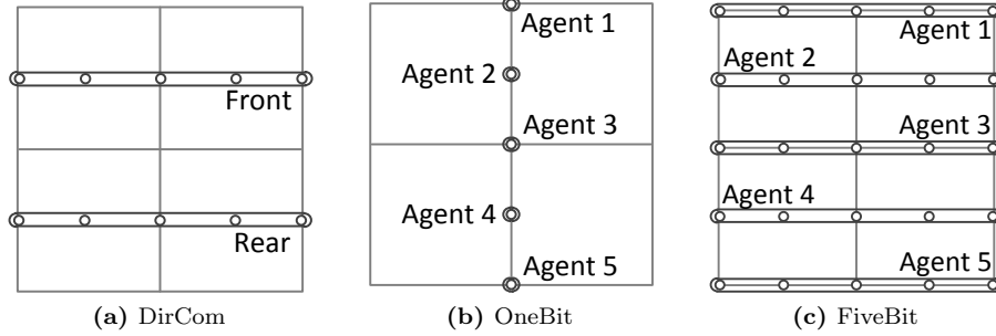
Figure 4: Substrate: communication input planes. Communication input for DirCom (a) consists of two sets of five neurons corresponding to the front and rear pie-slice sensors. Each neuron in the communication input plane for OneBit (b) corresponds to an agent on the team and is activated when detecting signals from that agent. The communication input plane for FiveBit (c) consists of a 5 \times 5 grid arranged as five horizontal groups. Each horizontal group corresponds to an agent on the team, and each neuron within a group corresponds to a different communication channel.
