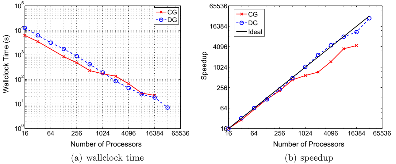
Fig. 10. Scaling study performed using the NUMA-CG and NUMA-DG codes for the RTB problem using 32^3 elements and N = 8 .
