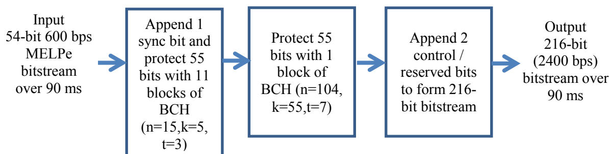
Fig. 18 — Frame-by-frame conversion from 600 bps MELPe mode to 600/2400 bps fixed rate mode
