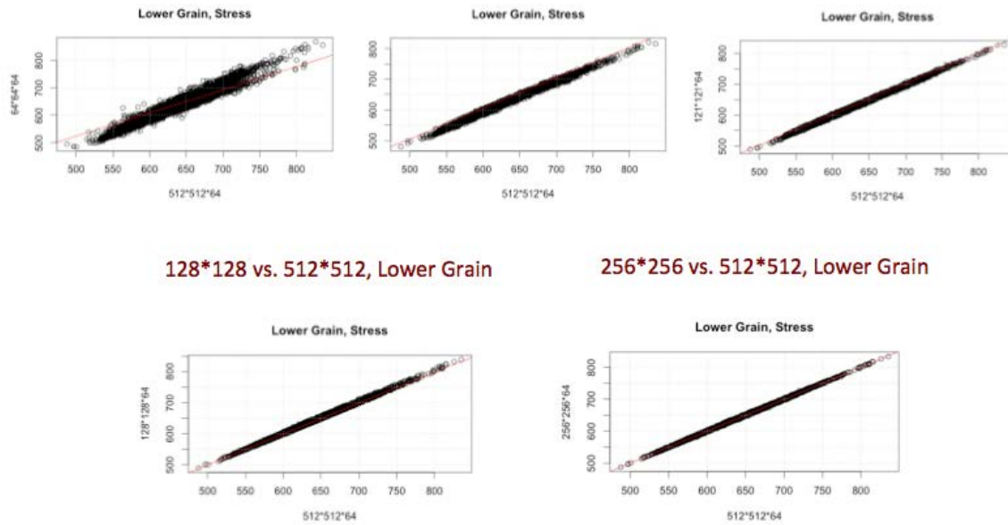
Figure 3.4. Correlation plots between the biggest RVE and others, for lower grain max principal stress values.
