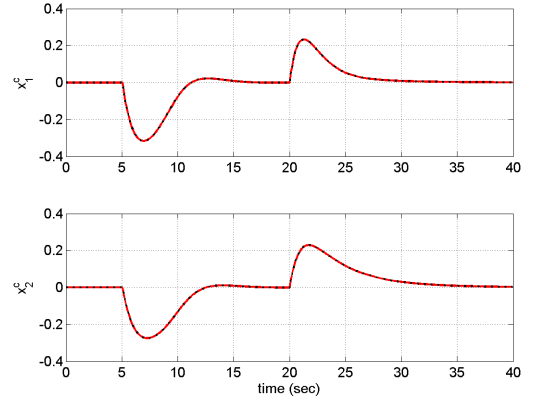
FIGURE 16. Controller states ( x^c )
