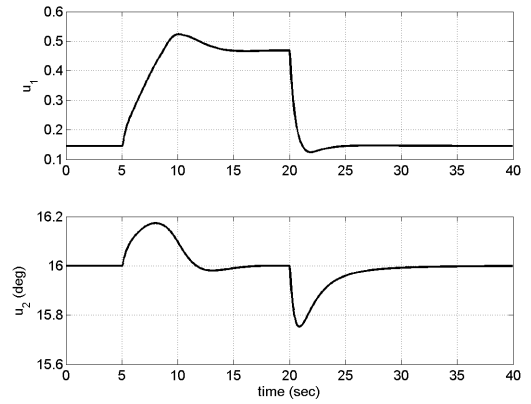
FIGURE 22. Fuel and prop pitch angle control inputs ( u(t) )
