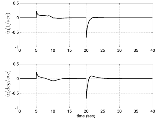
FIGURE 21. Rate of change for fuel and prop pitch angle control inputs ( \dot{u}(t) )
