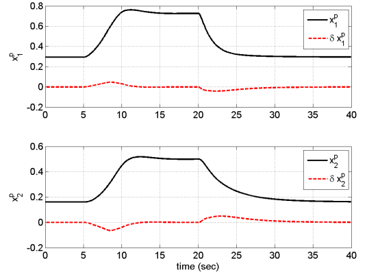
FIGURE 15. Plant states: high and low spool speeds ( x^p )
