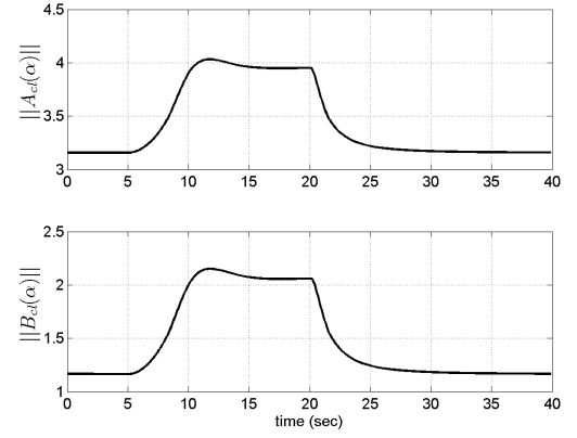
FIGURE 11. Norm of the closed-loop system matrices ( \|A_{cl}(\alpha)\| , and \|B_{cl}(\alpha)\| )
