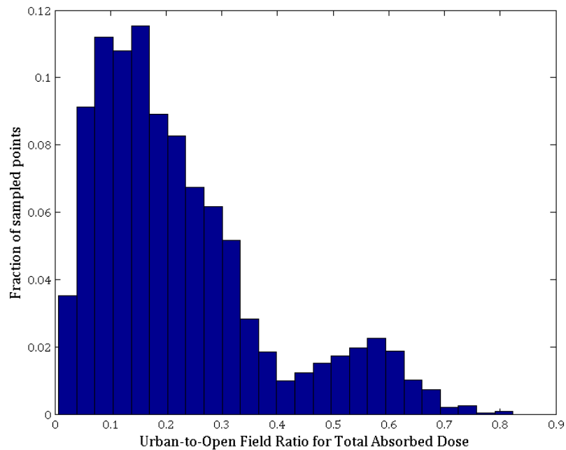
Figure 5-12. Variation of Urban-to-Open Field Total Absorbed Dose Ratio at 1200 m from detonation location
