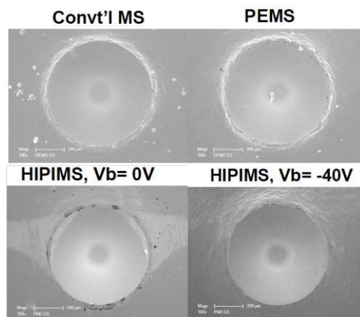
Fig. 6i Comparative Cr deposition using DCMS, PEMS, HIPIMS: Upper: Row 1- cross section, Row 2- topography, Row 3- AFM surface roughness. Left- RC indentation testing showing conventional DCMS deposited Cr has poor adhesion compared to PEMS and HIPIMS with and without bias.
