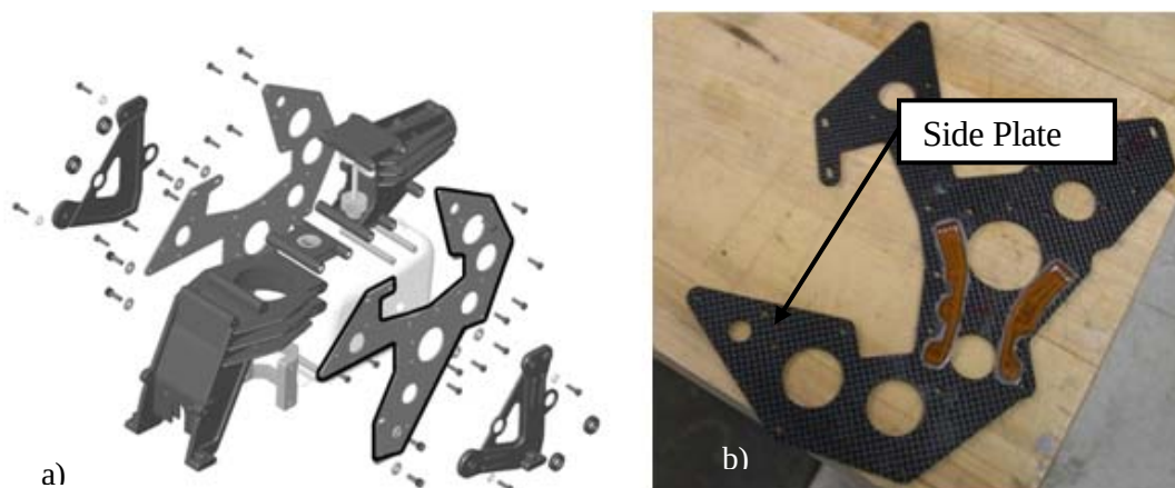
Figure 2: a) The Raptor 90 Airframe and Selected PSE b) The Side Plate with Sensors Installed
