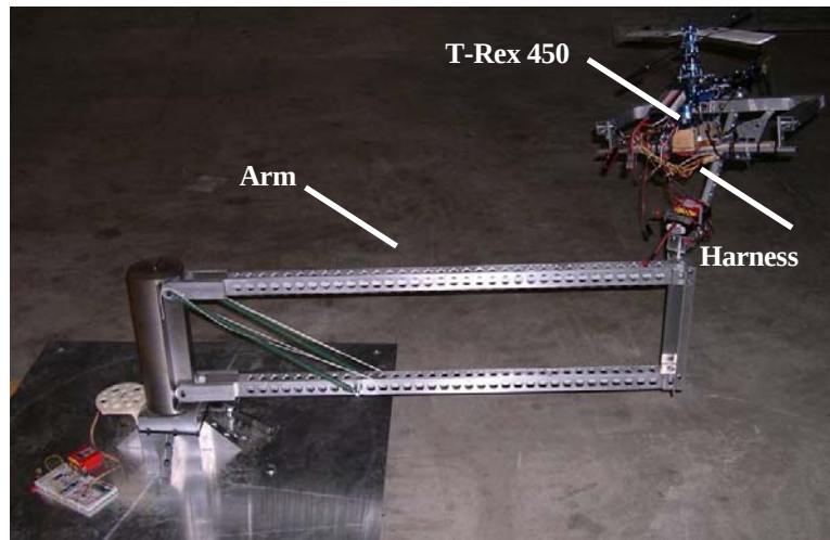
Figure 3: Ground-based Flight Test Stand with T-Rex 450
