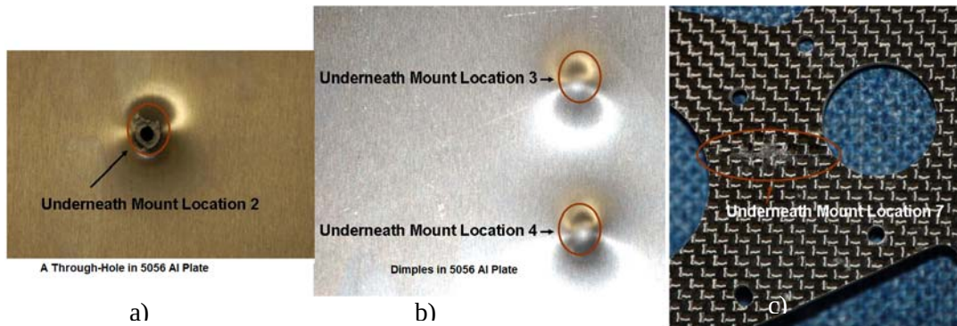
Figure 4: a) &amp; b) Underneath M100 Test on Flat Al 5056 Plates c) on Composite Raptor 90 Side Plate
