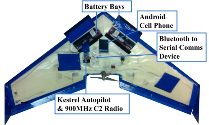
Figure 5: Modified Procerus Unicorn UAV
