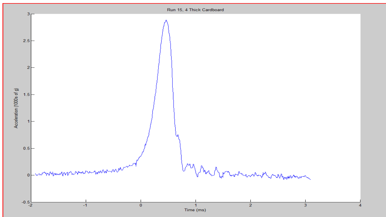
Figure 21. Trial 15: Four thick cardboard pieces.
