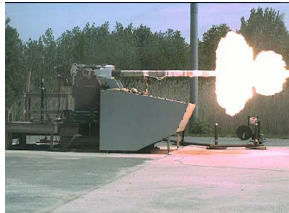
Figure 5. Test firing at APG
