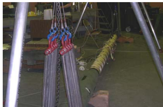
Figure 3. Modal testing setup.
