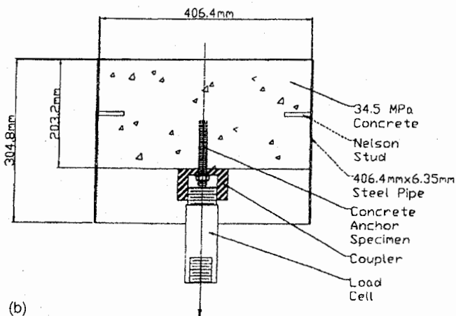
Fig. 7. Concrete anchor mount: (a) hole preparation; and (b) schematic test setup
