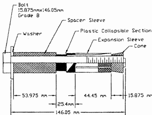
Fig. 3. Torque-controlled expansion anchor
