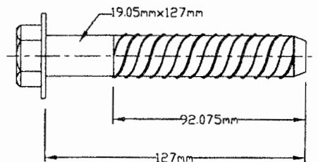
Fig. 6. Typical self-threading anchor
