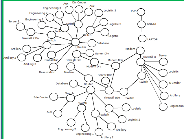
Core Simulation Manager (CSimMan)
