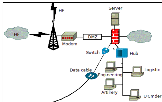
Figure 5 - IT Infrastructure at the Unit level
