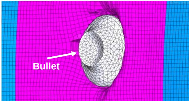
Figure 8. Final deformed shape of a defeated 9mm round-nose bullet
