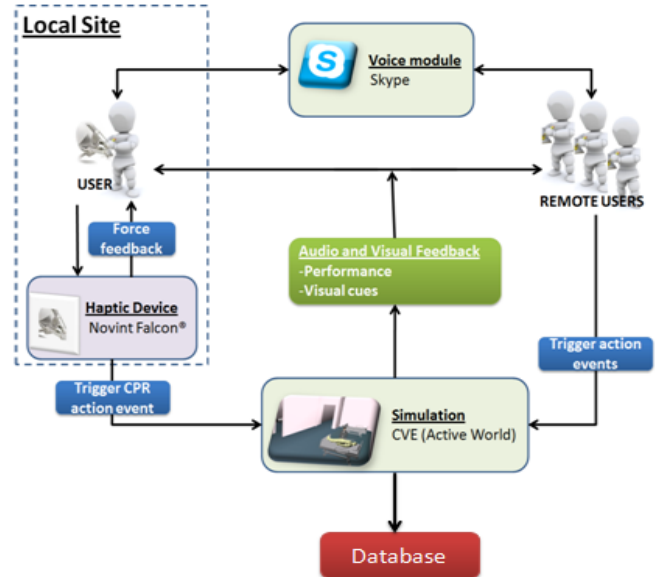
Figure 1. System Design.
