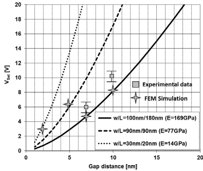
Figure 4.24. Calculated V_{\text{Set}} as a function of as-fabricated actuation gap thickness for scaled memory cells, for various values of Young's modulus E . Selected measured data and values obtained from finite-element-method simulations are also shown, to verify the accuracy of the analytical model.
