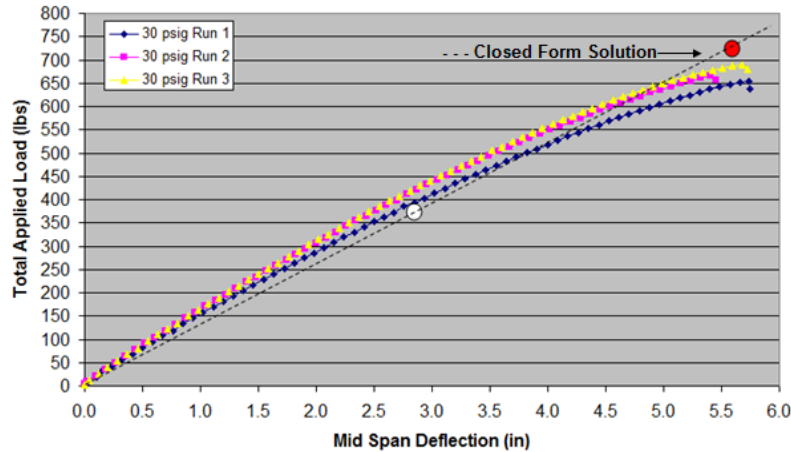
Figure 24. Load Versus Midspan Deflection for 30.0-psig Inflation
