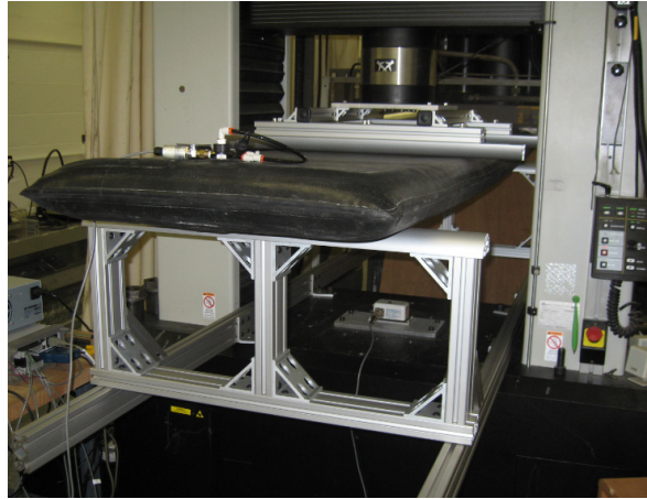
Figure 18. Experimental Four-Point Bend Test Arrangement
