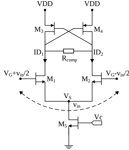
Fig. 10. Differential Transconductor
