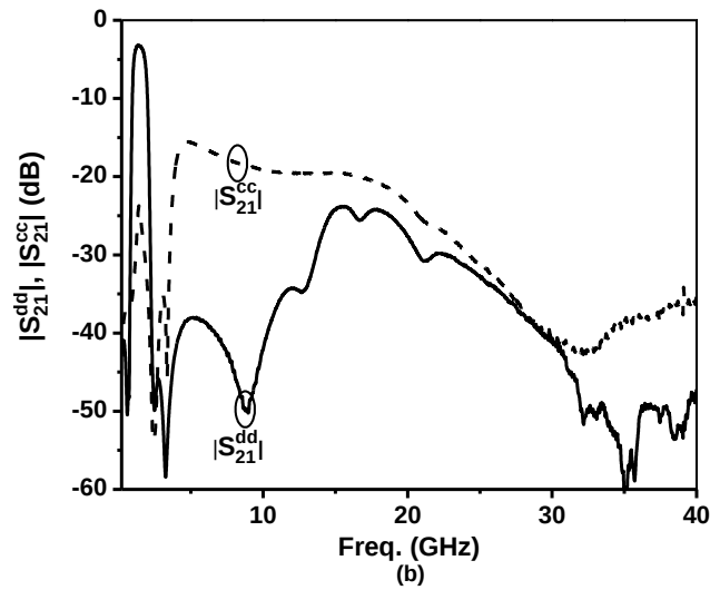
Fig. 7. (a) Simulated and measured results. (b) Measured results for a wider frequency range.
