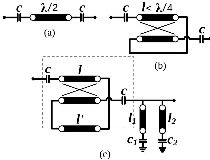
Fig. 18. (a) Half wavelength capacitively loaded resonator. (b) Coupled line capacitively loaded resonator. (c) Proposed filter using coupled line capacitively loaded resonator.
