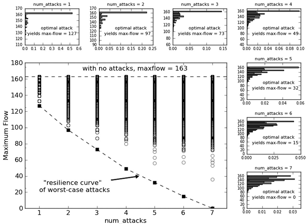
Figure 5. Random attacks on the Soviet Railway, compared with optimal ones. Maximum flow (system performance) degrades with an increasing number of damaged edges. For num\_attacks = 1, 2, \dots, 7 , we present the worst-case disruption, along with 10,000 randomly generated attacks. Each subfigure shows a histogram of the frequency with which random attacks impact the maximum flow. As the number of possible attack combinations increases, it becomes harder and harder to find the worst-case attack by random sampling. In the main figure, the dashed line connects the worst-case disruptions for this system. (Here the phrase “resilience curve” really refers to a discrete frontier of points.)
