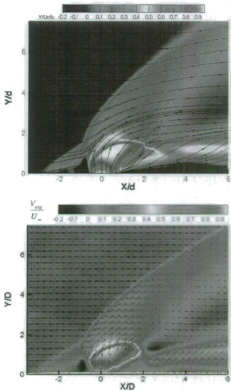
Figure 4. Contours of normalized mean wall-normal velocity. Simulation upper, experiment 16 lower.
