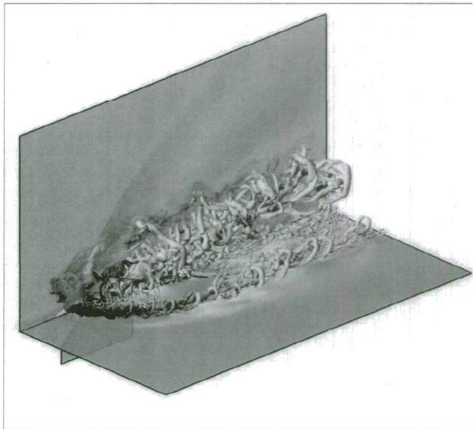
Figure 7. Isosurfaces of Q -criterion; temperature contours.
