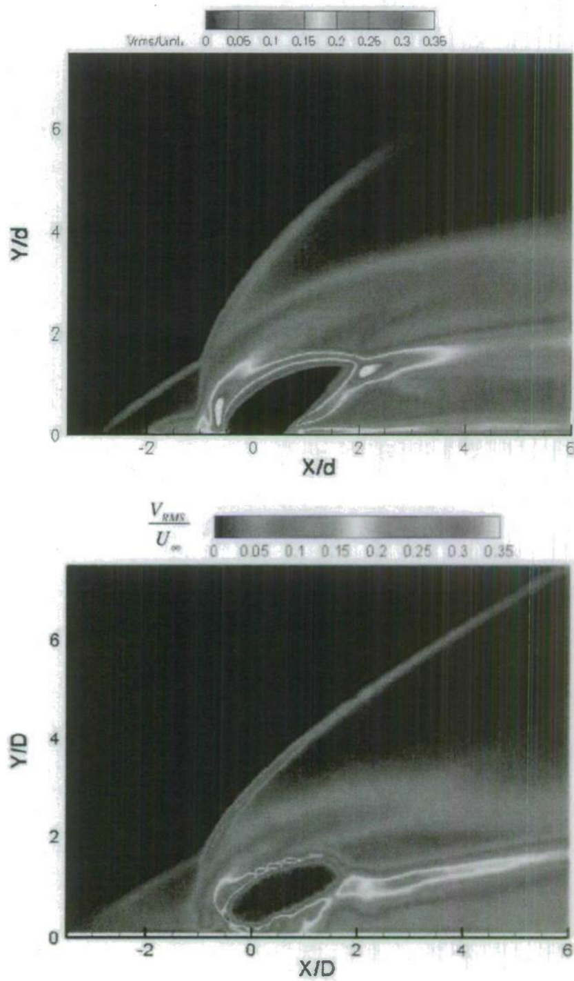
Figure 6. Contours of normalized RMS wall-normal velocity. Simulation upper, experiment 16 lower.
