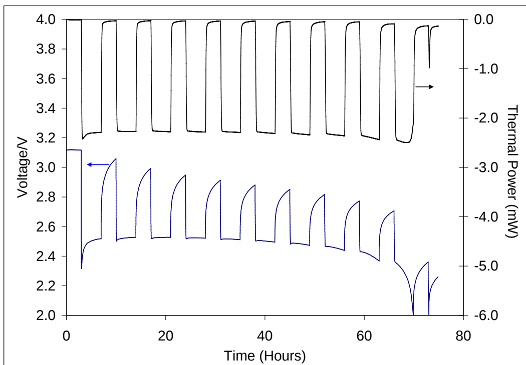
Figure 2. Li-CFx cell voltage and thermal power (mW) versus time for 20 mA/g discharge rate.
