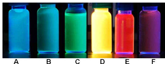
Fig. 11. Photo taken under the 365 nm UV radiation with different color emitting InP/ZnS QDs prepared from indium acetate (4 mmol) and tris(trimethylsilyl)phosphine (8mmol) at 178 °C; (A) \lambda_{em} = 492 nm, (B) 505 nm, (C) 526 nm, (D) 604 nm, (E) 632 nm, (F) 809 nm.
