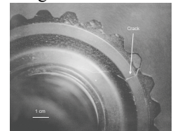
Figure 10. IGB crack. The crack growth test consisted of rotation in a spin pit, at a constant high speed with a varying load cycle, to simulate flight conditions. Data collection was done using 2 stud mounted accelerometers at the input and the output of the IGB.
