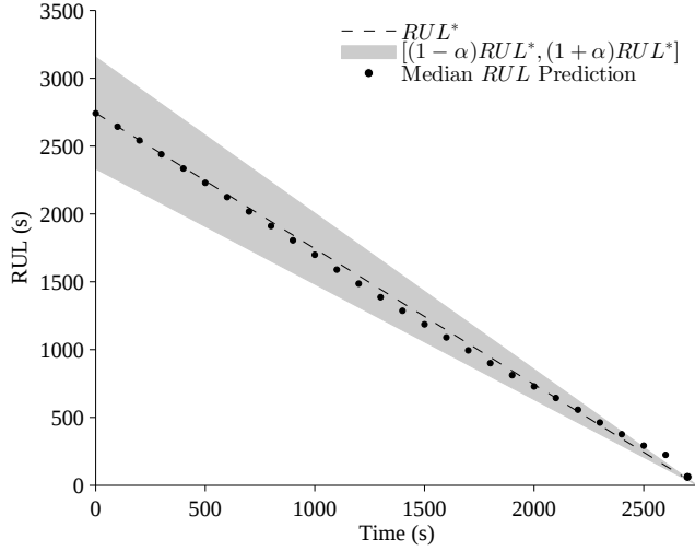
Figure 5. Prediction performance assuming known future input trajectory and no process noise with \alpha = 0.15 .
