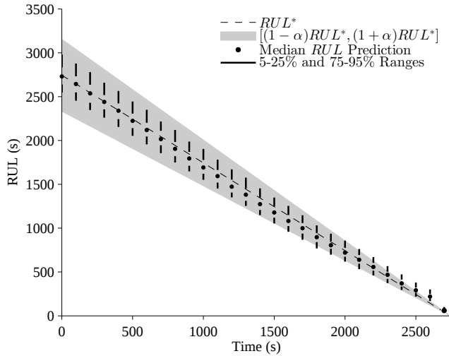
Figure 6. Prediction performance assuming known future input trajectory and 100 process noise samples with \alpha = 0.15 .
