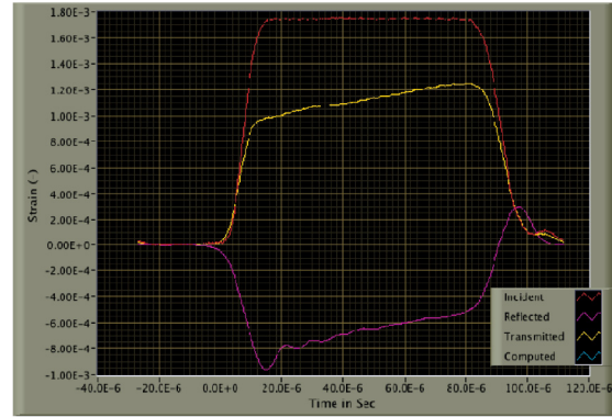
Fig. 4. Aluminium Al 6061-T6 tested with undamaged bars.
