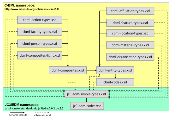
Figure 4- SISO C-BML Phase 1 Schema Structure
