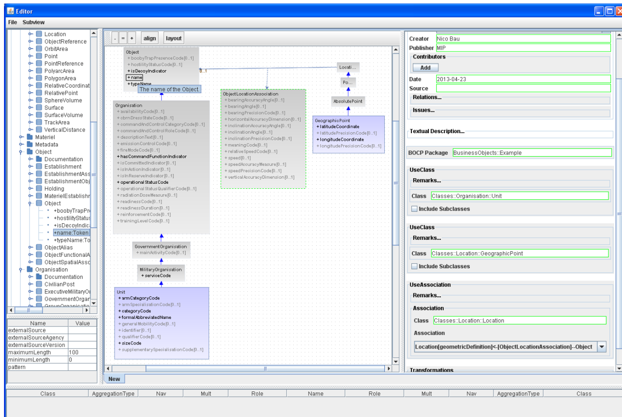
Figure 7-MIP Model Editor
