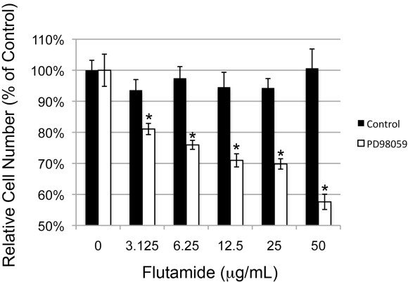
Fig. 9: A flux in the mevalonate-to-Ras pathway, generated from the depletion of the mitochondrial genome content, in PCa advances the disease to the AAR phenotype. Depicted is a graph of the viability of LNp0-8 that was seeded at a concentration of 2,000 cells/well in a 96 well plate, overnight. Cells were cultured 4 days in the absence or presence of flutamide at the denoted dosage. Cells cultures were additionally supplemented without (control) or with 40 µM PD98059 (n = 3). After treatment, the viability of cells was quantified in a calcein assay and the mean of each group was reported as a relative percent to the control, 0 µg/mL Flutamide (arbitrary unit ± SE). A student's t-test was conducted to compare the viability of cells exposed to control and PD98059 conditions in the same dosage of flutamide (*p < 0.001). Error bars represent standard error.
