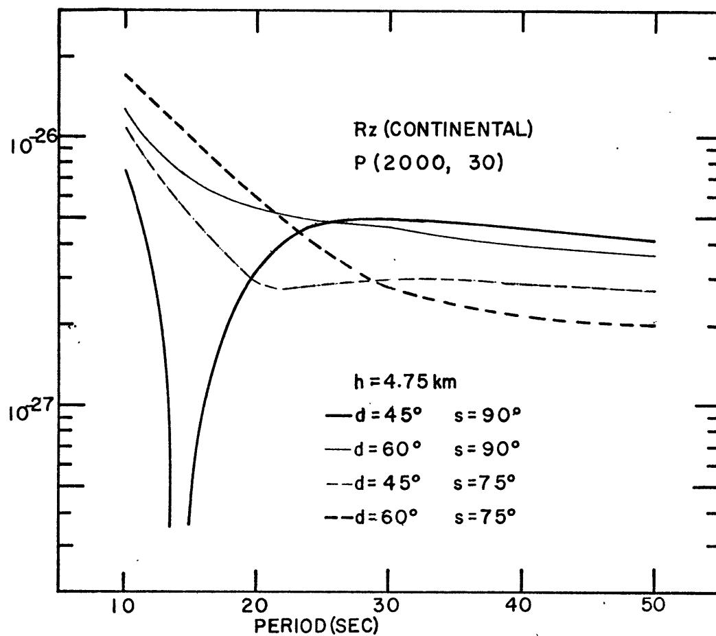
FIG. 16. Variations of the Rayleigh wave amplitude spectrum due to 15 degree change in the dip or/and slip angles of a dip-slip fault at depth 4.75 km.
