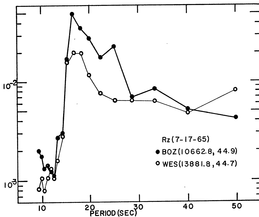
FIG. 26c. Rz amplitude spectrum at BOZ and WES.
