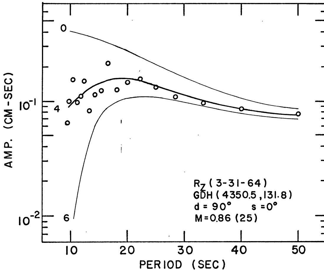
FIG. 44. R_z from event P14 observed at GDH.
