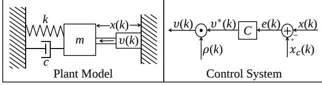
Figure 2. Diagram of mass-spring-damper plant model and control system
