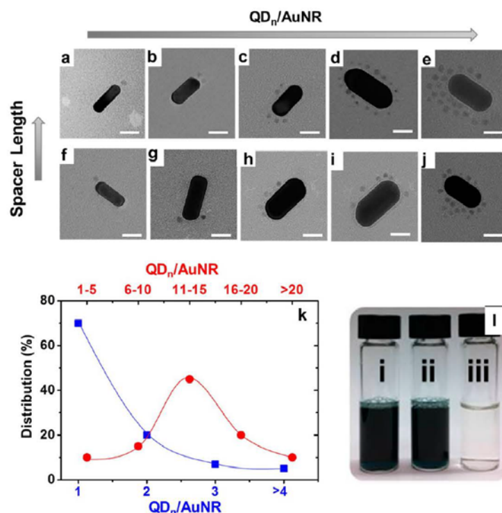
Figure 2. Structural control of QD-AuNR assembly in aqueous solution. TEM images (scale bar = 25 nm) showing control of spacing, position and QD_n/AuNR ( n is the number of QD per AuNR). Spacing length is controlled by changing ligand length [AUT (a–e), AHT (f–j)]. Ligand position and QD_n/AuNR is controlled by incrementing QD concentration from 0.2 (a,b,f,g), 0.5 (c,h), 1.5 (d,i), 2.5 nM (e,j) at 0.2 nM AuNR concentration. (k) Distribution of QD_n/AuNR in the reaction solution with 0.2 nM QD (blue) and 2.5 nM QD (red) (the lines for clarity only). (l) Picture of vials containing aqueous solutions of (i) AuNR (0.7 nM), (ii) QD_n/AuNR (product from 0.7 nM AuNR and 1.4 nM QD), and (iii) QD (1.4 nM).
