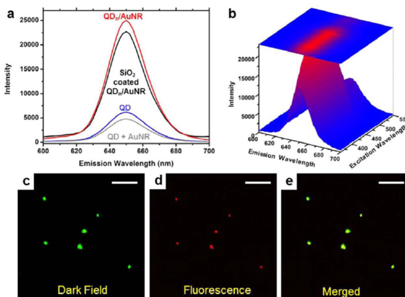
Figure 4. Photophysical properties of \text{QD}_n/\text{AuNR} in aqueous solution and on glass surface. (a) Photoluminescence spectra of aqueous solutions of equimolar QD concentration (0.4 nM): \text{QD}_n/\text{AuNR} ( n = 3 \pm 1 , in which >50% of QD are at AuNR ends) (Red); its silica encapsulated product (Black); base mixture of QD (0.4 nM) and AuNR (0.2 nM) in the absence of AUT spacer (Gray); and control QD (absence of AuNR) (Blue). (b) A combination of 2D and 3D counter plot of PL spectra of \text{QD}_n/\text{AuNR} acquired at different excitation wavelength from aqueous solution showing an emission maximum at 650 nm. Bottom images are obtained from dark field hyperspectral imaging microscope using dual imaging modalities of \text{QD}_n/\text{AuNR} architectures spread between two glass coverslips. (c) Dark field scattering (570 nm excitation). (d) Fluorescence emission (570 nm excitation; fluorescence collected at 610 nm with long pass filter). (e) Merged image of (c) and (d) showing overlap of signals confirming the sample purity. The scale bars are 10 \mu\text{m} .
