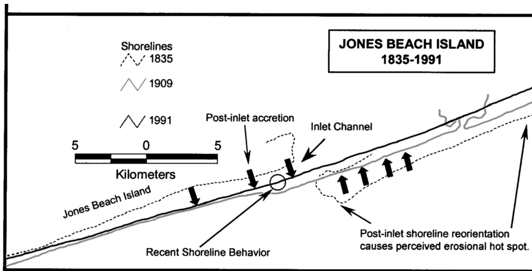
Figure 6. Evolution of Jones Beach Island, Long Island, NY, a relict inlet
