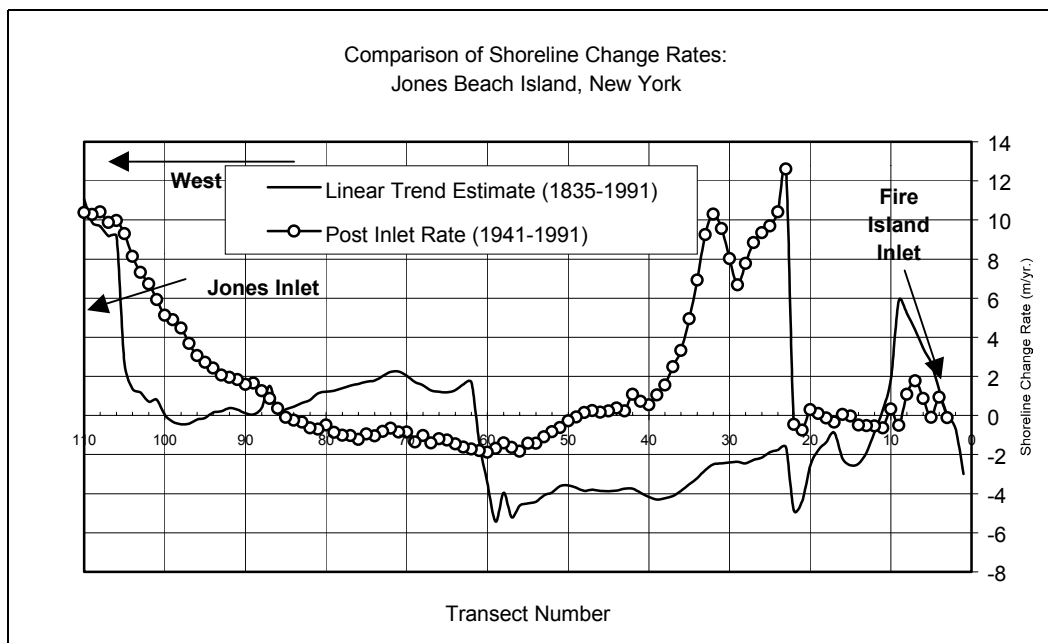
Figure 7. Shoreline change rates, Jones Beach Island, NY
