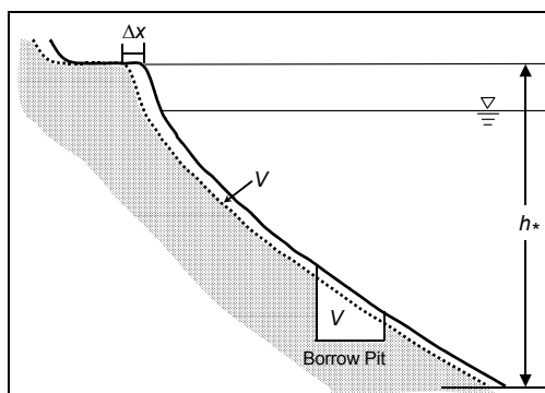
Figure 3. Definition sketch for borrow site located on active profile
