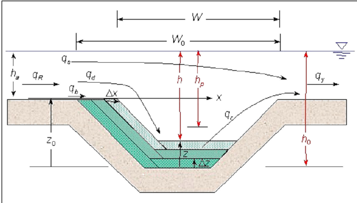
Figure 2. Definition sketch for channel infilling model
