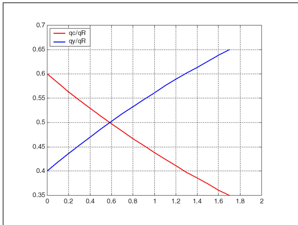
Figure 5. Evolution of channel infilling rate and channel bypassing rate on sand shore
