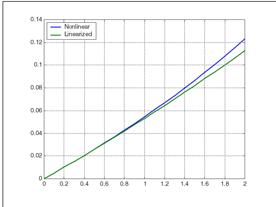
Figure 6. Increase in elevation (decrease in depth) in channel on gravel shore: comparison of nonlinear model (numerical solution) and linearized model (analytical solution)
