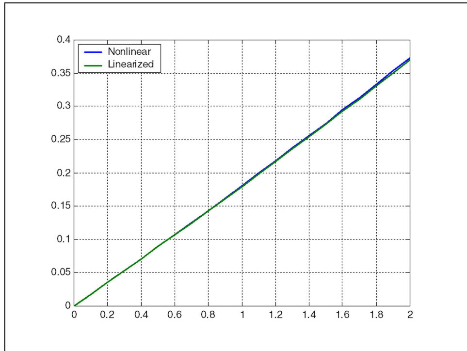
Figure 7. Increase in intrusion distance (decrease in width) in channel on gravel shore: comparison of nonlinear model (numerical solution) and linearized model (analytical solution)
