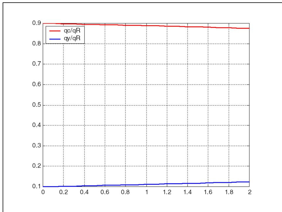
Figure 8. Evolution of channel infilling rate and channel bypassing rate on gravel shore
