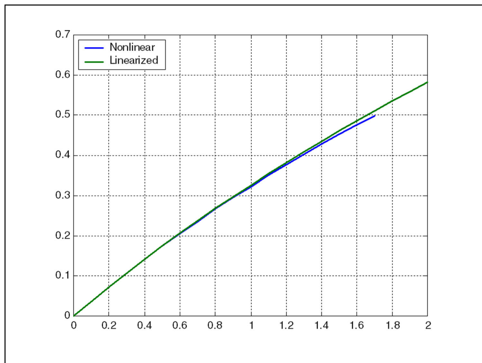
Figure 3. Increase in elevation (decrease in depth) in channel on sand shore: comparison of nonlinear model (numerical solution) and linearized model (analytical solution)
