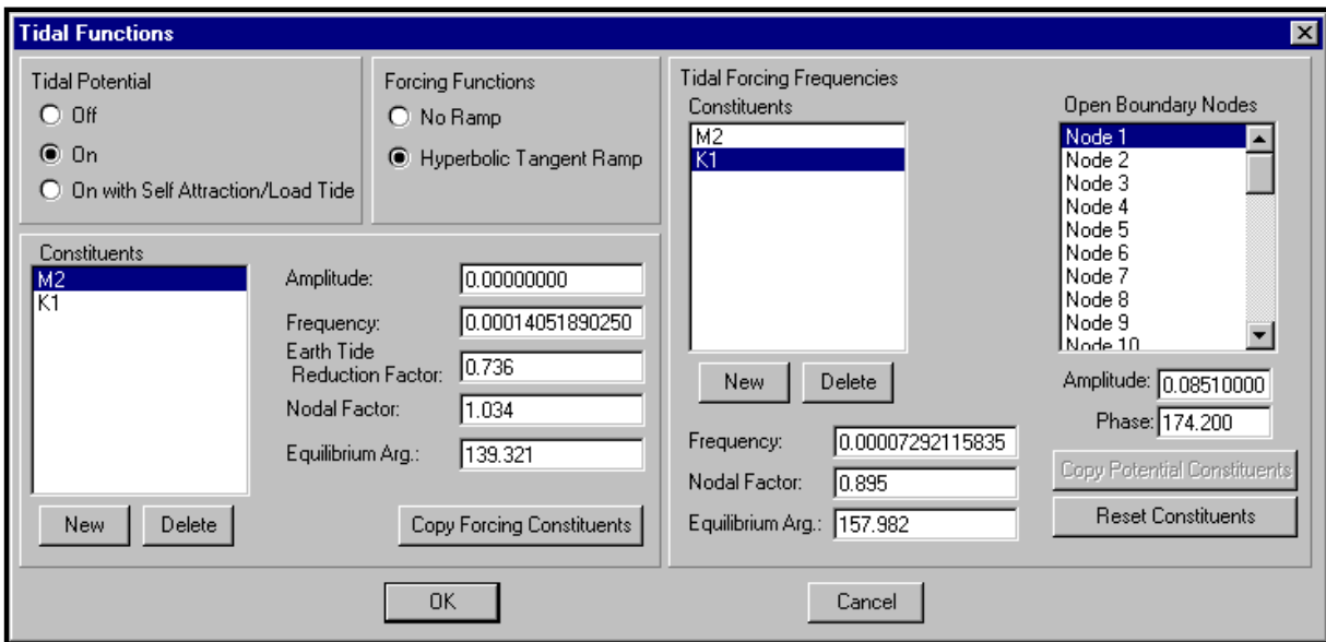
Figure 7. Tidal Functions dialog box with M2 and K1 constituents selected
