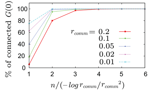
Fig. 9. Effects of n on the connectivity of G(0) for different values of r_{\text{comm}} .
