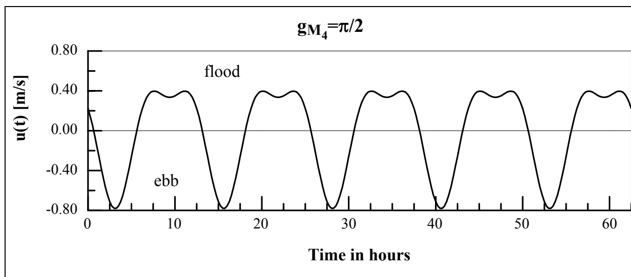
b. Channel velocity vs. time (phase lag = 90 deg)
