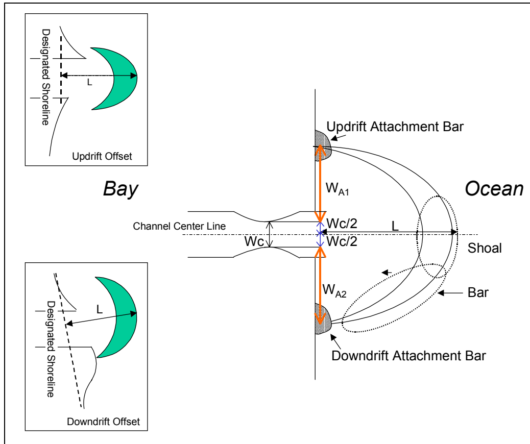
Figure 2. Symmetric ebb shoal with definitions of terminology used in measurements
